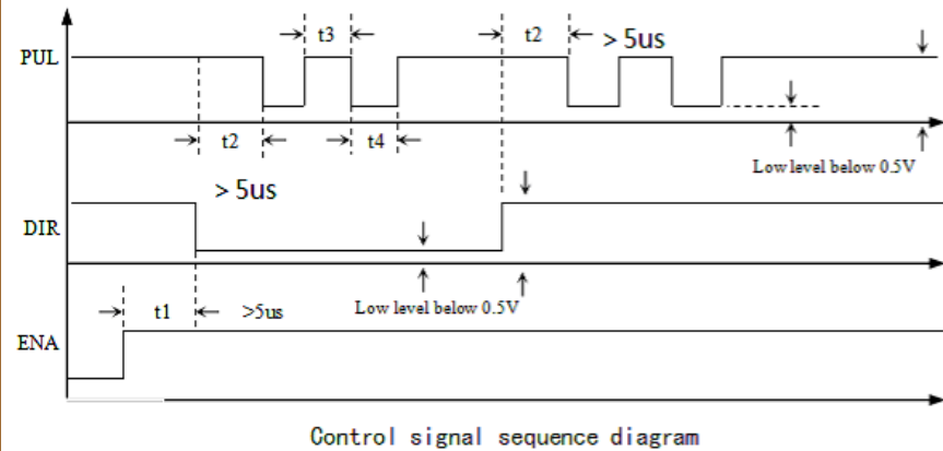
Control Signal Sequence Diagram
